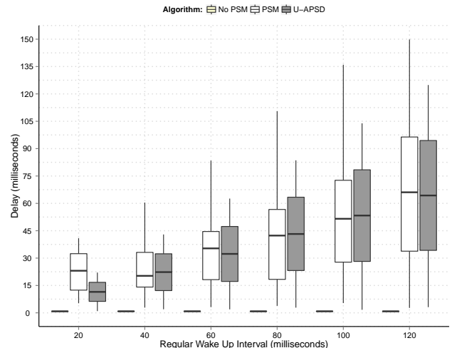
Fig. 2. End-to-end delay for distinct wake up periods
