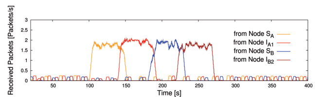
Fig. 3: MaxMAC: Packet Reception Rate from Nodes S_A , I_{A1} , S_B and I_{B1} .
