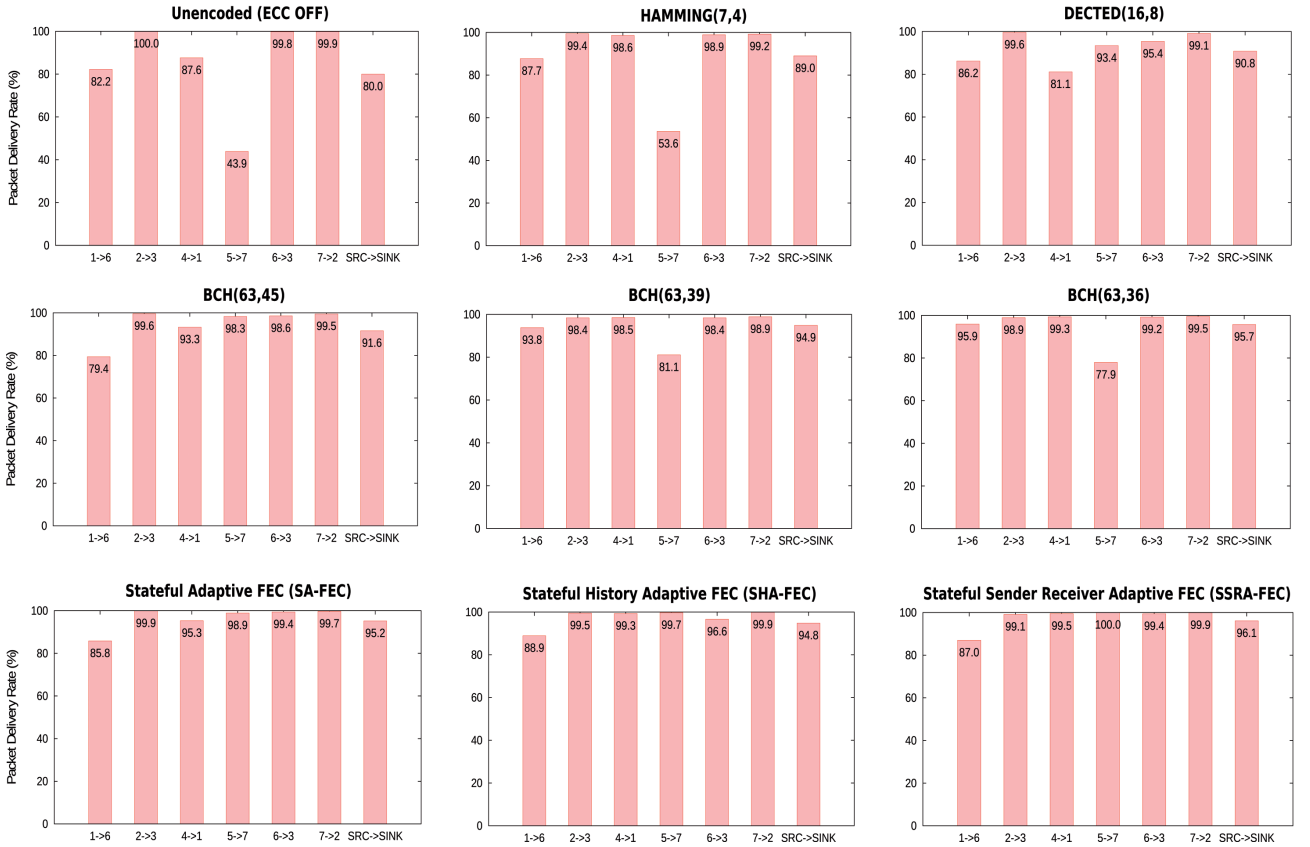
Fig. 7: PDRs per Link and Overall Source-to-Sink PDR.
