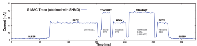
Fig. 5: Current Draw of physically measured node.
