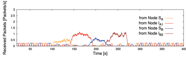
Fig. 4: WiseMAC: Packet Reception Rate from Nodes S_A , I_{A1} , S_B and I_{B1} .
