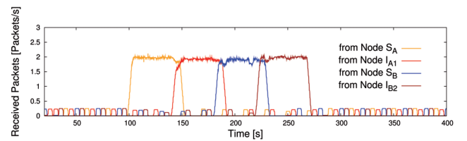
Fig. 2: CSMA: Packet Reception Rate from Nodes S_A , I_{A1} , S_B and I_{B1} .
