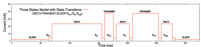
Fig. 6: Current Draw as modeled by our software-based energy estimation basing on the Three States Model with State Transitions .
