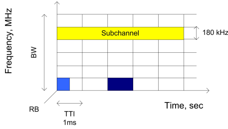
Fig. 2. LTE radio resource structure.
